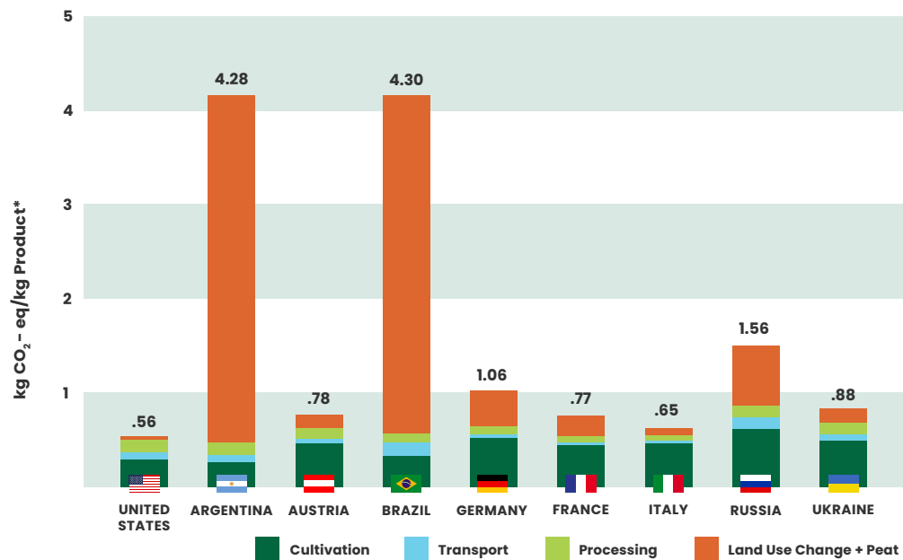
Figure 4. Shows the carbon footprint of soybean meal for the European market, including land use change, across various sourcing countries.
