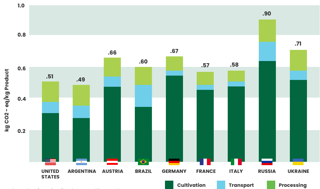
Figure 3. Illustrates the carbon footprint of soybean meal imported from various countries for the European market.
