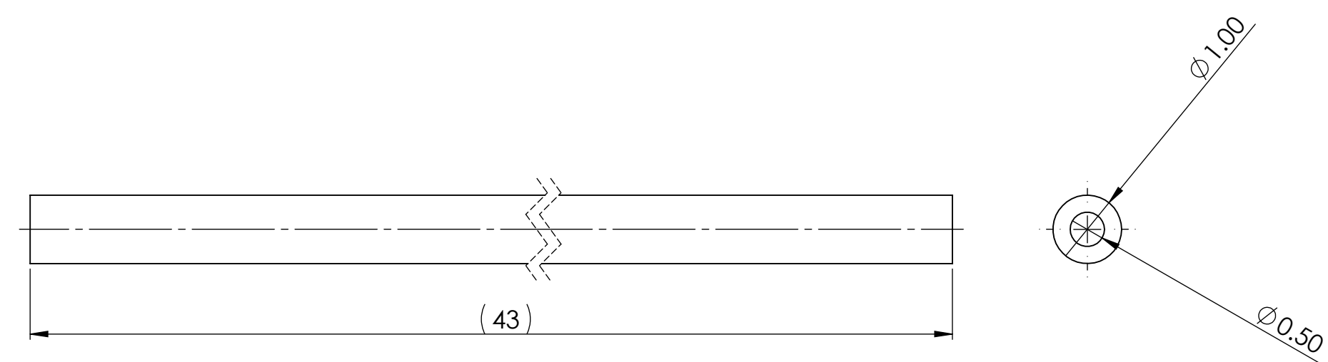
ITEM NO.-4 DIFFUSER TUBE-PERFORATED SCALE 1 : 2
