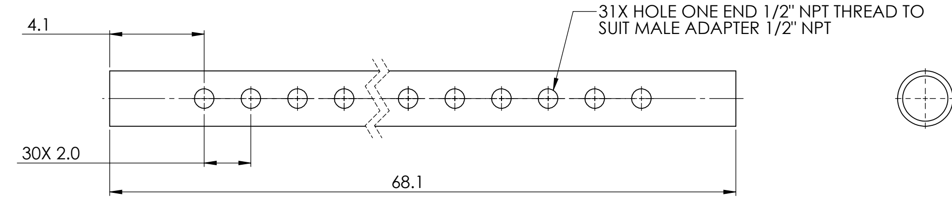
ITEM NO.-1 PIPE 2" PVC SCH80 SCALE 1 : 4
