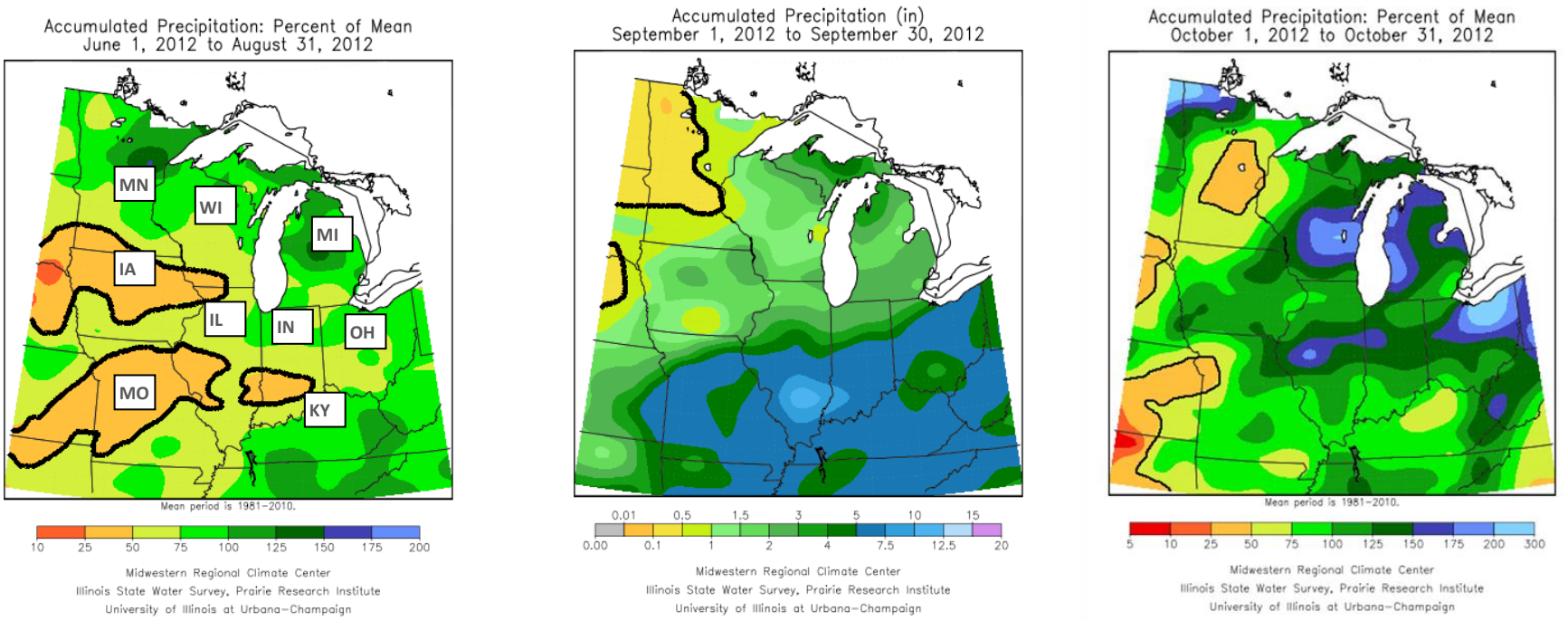
Figure 3. Areas outlined in black received less than 50% of average precipitation for the months indicated.
